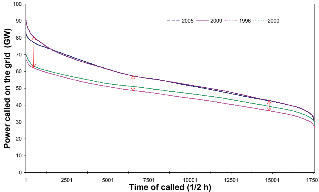
Figure 1: Power loaded on the grid (net demand) as a function of time (8 760 hours)
